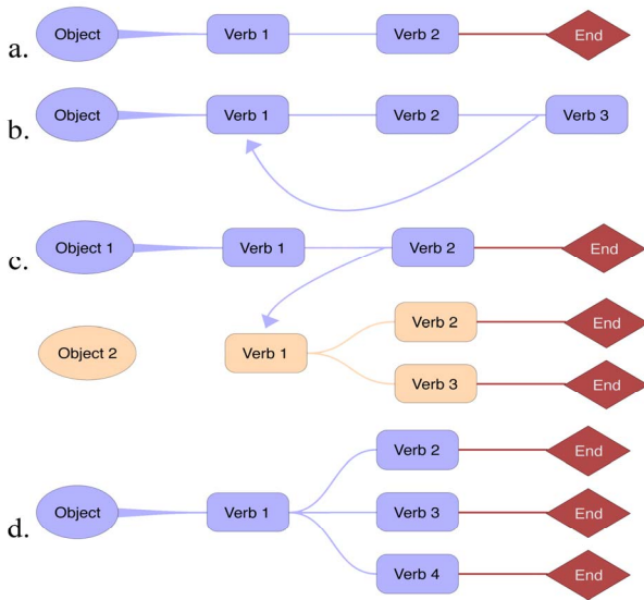
Fig. 2. Examples of the different structures of verb chaining that users can create
